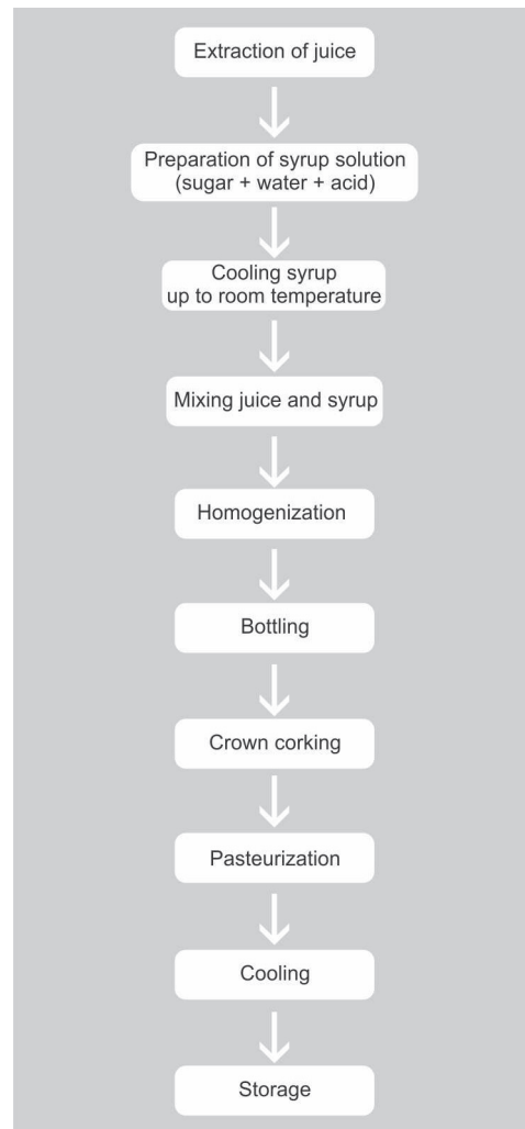
Figure 3. Flow sheet for preparation of ready-to-serve (RTS) aonla product.
